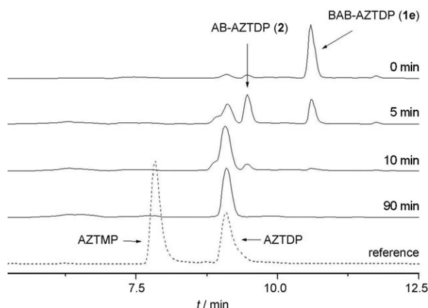
Figure 1. HPLC traces for BAB-AZTDP ( 1e ) after incubation in CEM/0 cell extracts for the time shown (0–90 min).
