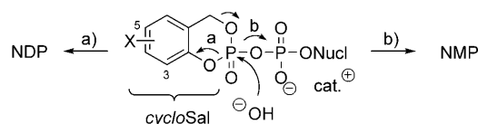
Scheme 1. Hydrolysis of cycloSal NDP prodrugs by paths a and b. ONucl = nucleoside.
