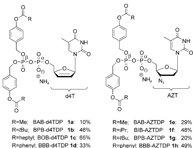
Scheme 3. Combination of the nucleosides and acyl moieties in prodrugs 1a–h . BAB = bis(4-acetoxybenzyl), BPB = bis(4-pivaloyloxybenzyl), BIB = bis(4-isobutyryloxybenzyl), BOB = bis(4-octanoyloxybenzyl), BBB = bis(4-benzoyloxybenzyl).
